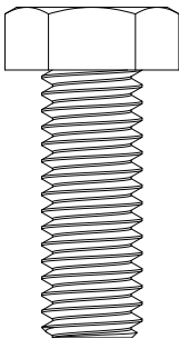
3/8"-16 Thread Size, 1" Long Hex Head Screw
